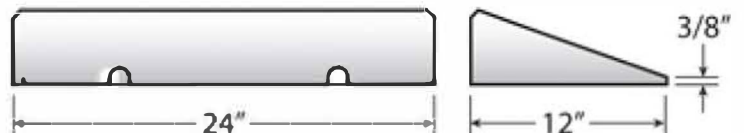
Side view 3.5" and 3.75" thick tile and ramp
